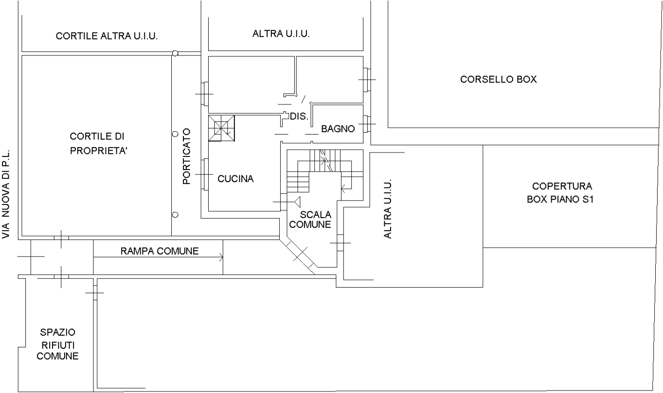
PIANO TERRA h = 2.70 m
